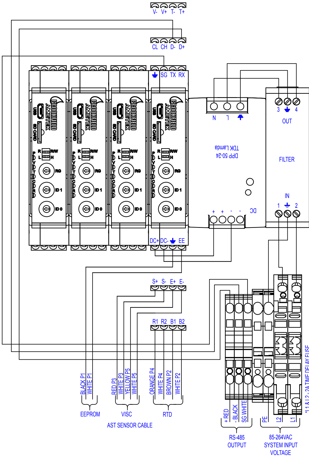
Figure B-2: 3-4 Unit MXT Enclosure Wiring Schematics
